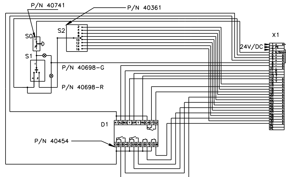
PROGRAMABLE TIMER ELECTRICAL SCHEMATIC
