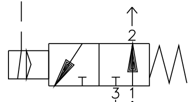
SOLENOID PLUMBING DETAIL
