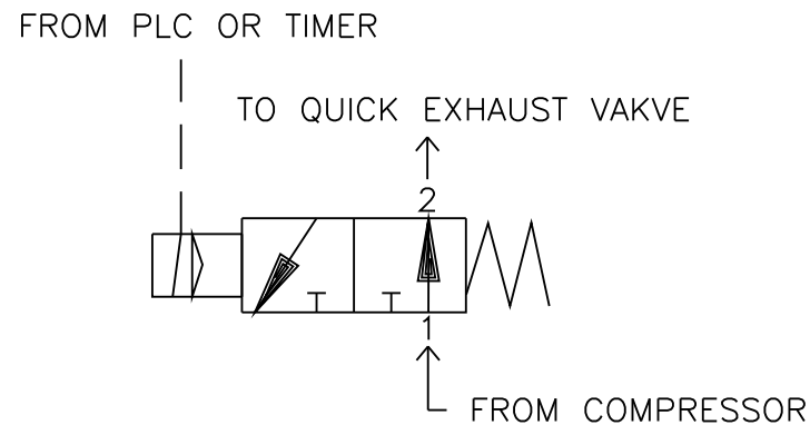
SOLENOID PLUMBING DETAIL
