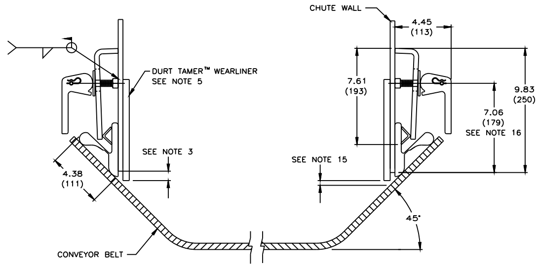
DETAIL FOR 45° BELT
