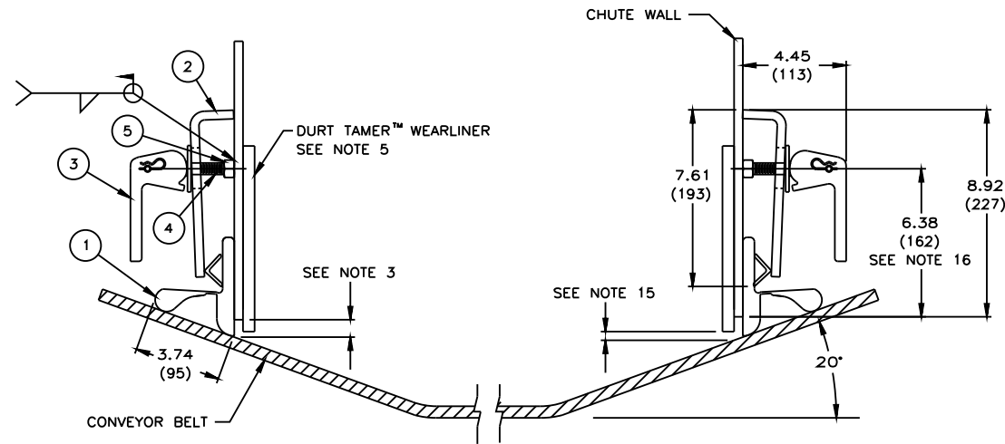
DETAIL FOR 20° BELT
