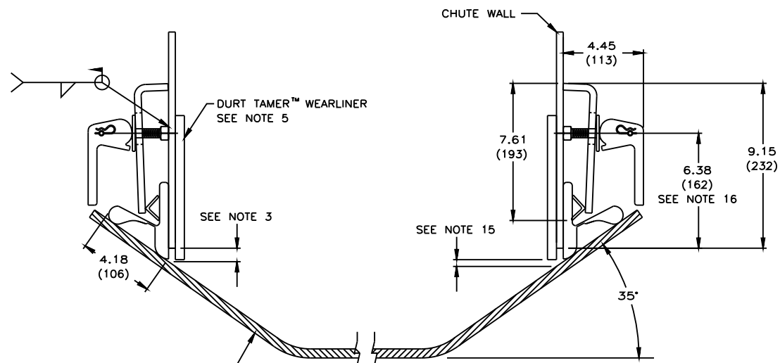
DETAIL FOR 35° BELT
