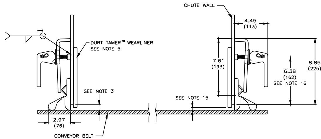
DETAIL FOR FLAT BELT
