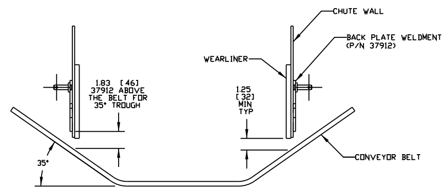
35° BELT LAYOUT SCALE 3/16
