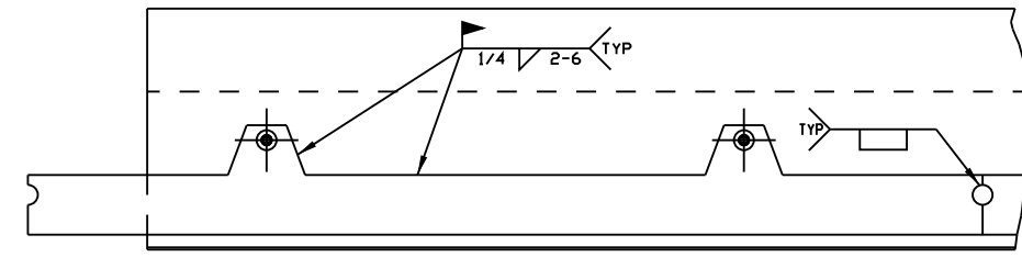
WELD DETAIL BELT NOT SHOWN FOR CLARITY
