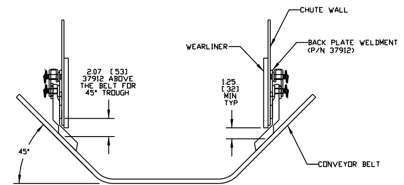
45° BELT LAYOUT SCALE 3/16
