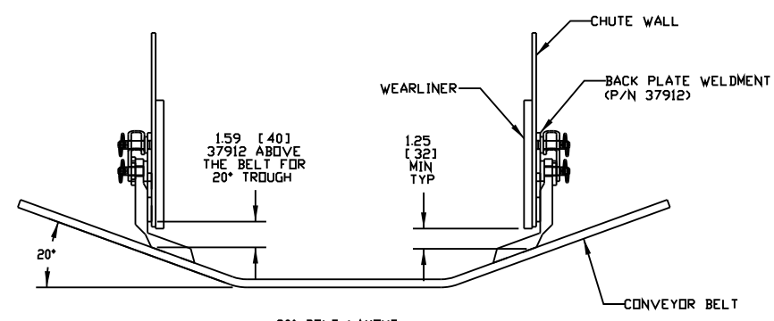
20° BELT LAYOUT SCALE 3/16
