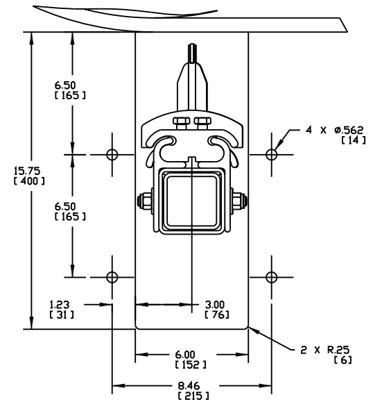
FAR SIDE CHUTE CUTOUT DETAIL SCALE 9/32
