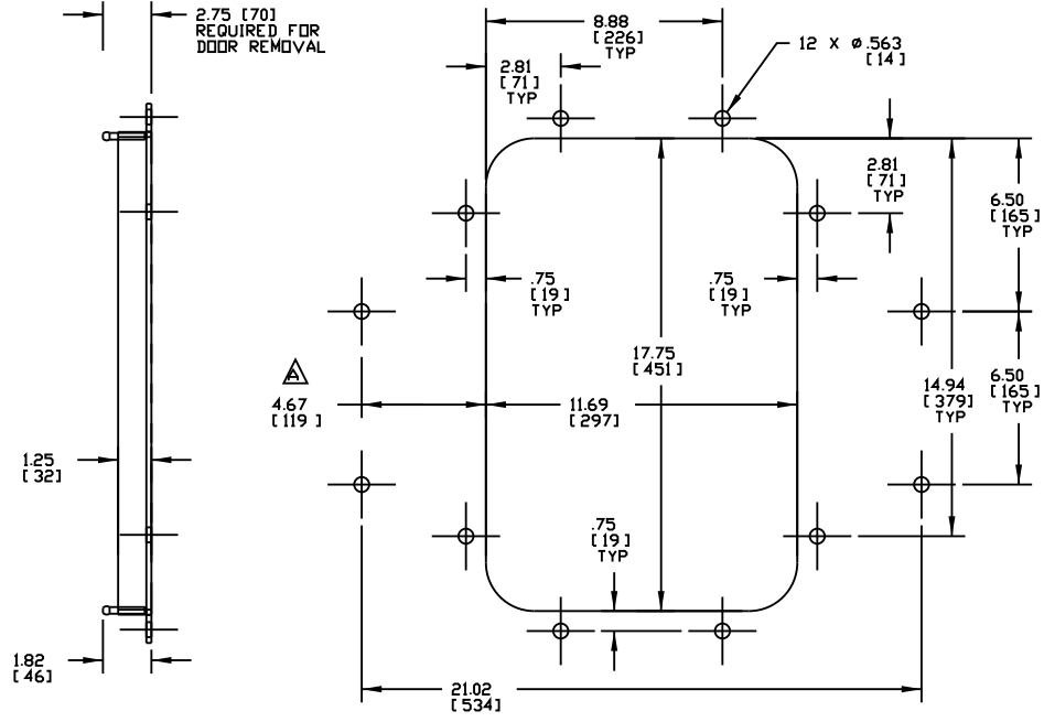
OPERATORS SIDE CHUTE CUTOUT DETAIL SCALE 1/4
