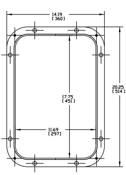
12.00 X 18.00 ACCESS DOOR DETAIL SCALE 1/4
